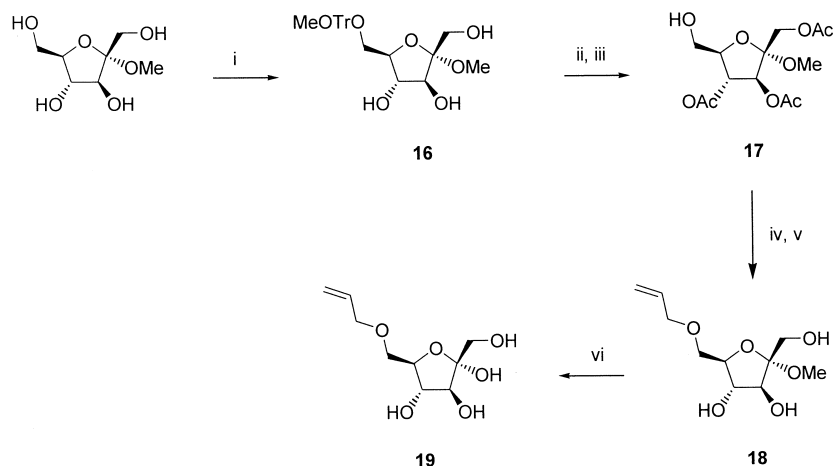
Scheme 4. Reagents and conditions: (i) (MeOPh) 3 CCl, pyridine, 4 °C; (ii) Ac 2 O, pyridine, 4 °C; (iii) AcOH; (iv) allylethylcarbonate, Ph 2 P-C 4 H 8 -PPh 2 ; (v) MeONa, MeOH; (vi) dioxane, 0.5M HCl.
