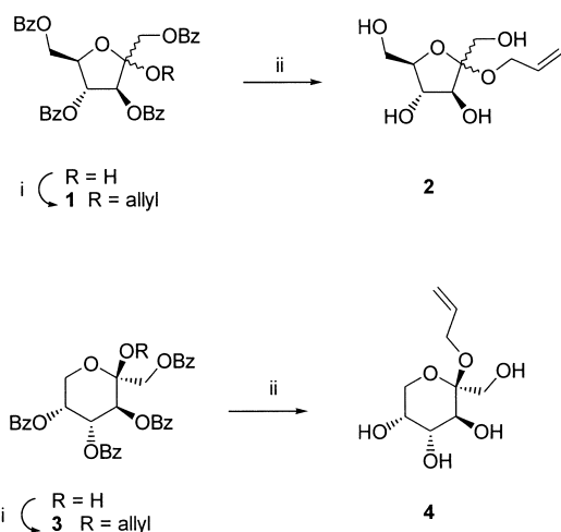
Scheme 1. Reagents and conditions: (i) allylmethylcarbonate, \text{Pd}_2(\text{dba})_3 , \text{Ph}_3\text{P} ; (ii) \text{MeONa} , \text{MeOH} .
