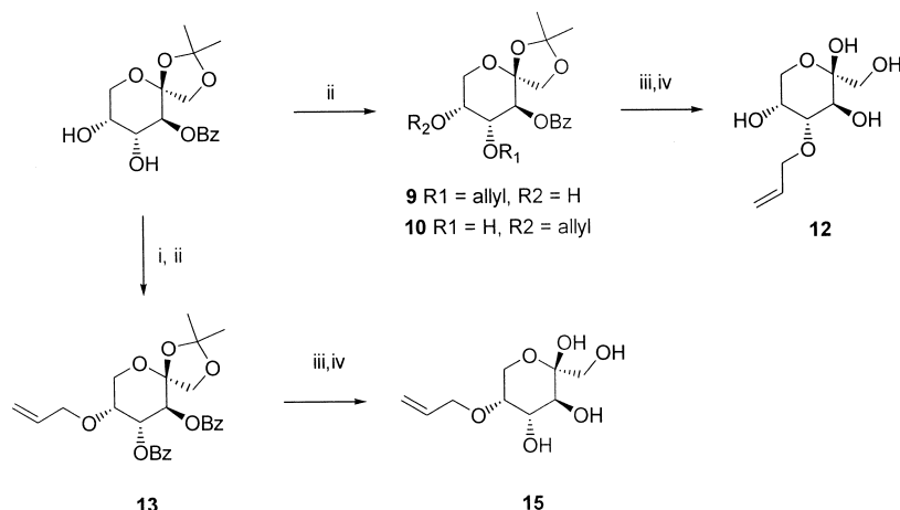
Scheme 3. Reagents and conditions: (i) \text{BzCl} , pyridine; (ii) allylmethylcarbonate, \text{Pd}_2(\text{dba})_3 , \text{Ph}_3\text{P} ; (iii) \text{MeONa} , \text{MeOH} ; (iv) \text{TFA-H}_2\text{O} (4:1).
